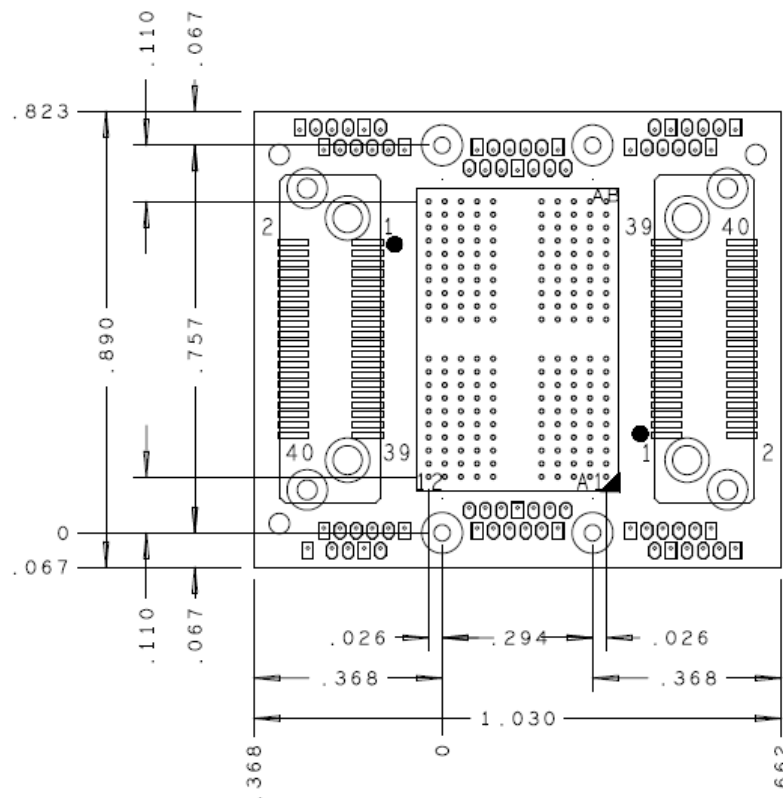
Figure 2 LPDDR4 200 Ball Compliance Interposer Mechanical Dimensions
