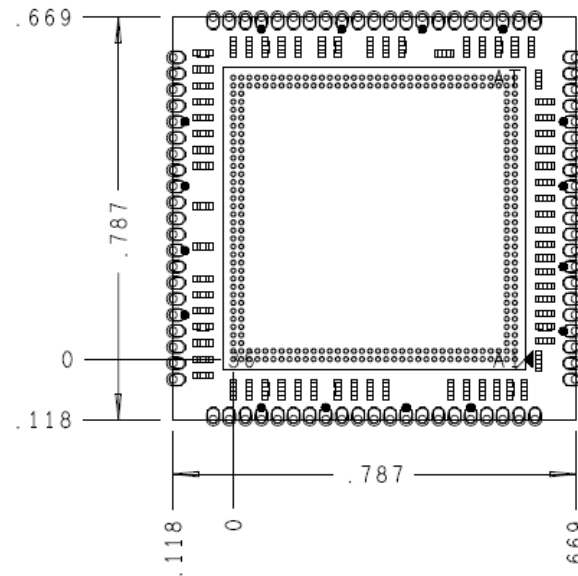
Figure 2 LPDDR4 272 Ball EdgeProbe Interposer Mechanical Dimensions
