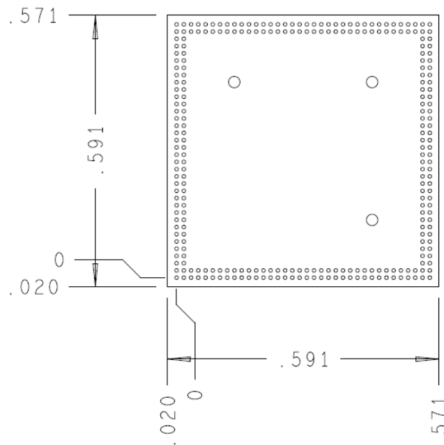
Figure 3 LPDDR4 272 Ball Riser Mechanical Dimensions
