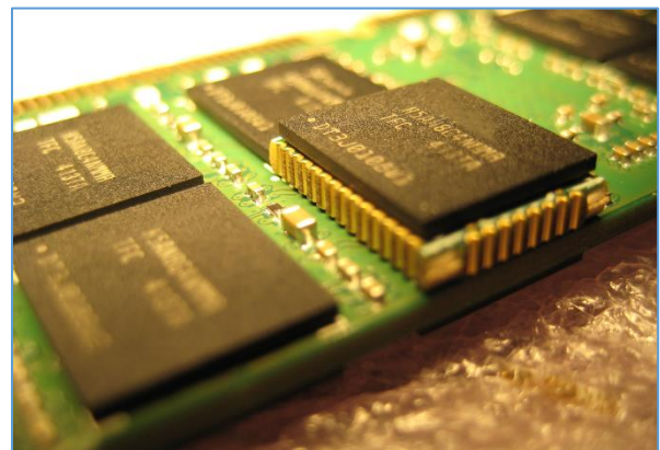
Figure 1 EdgeProbe interposer installed under a memory component
