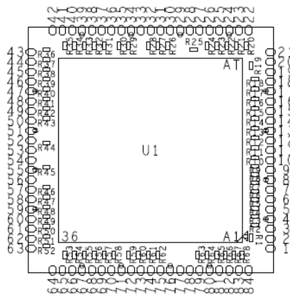
Figure 4 LPDDR4 272 Ball Edge Probe Probe Point Locations
