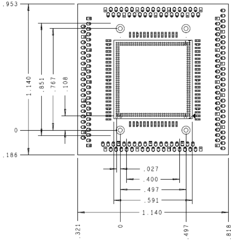
Figure 2 LPDDR4 272 Ball Direct Attach Interposer Mechanical Dimensions
