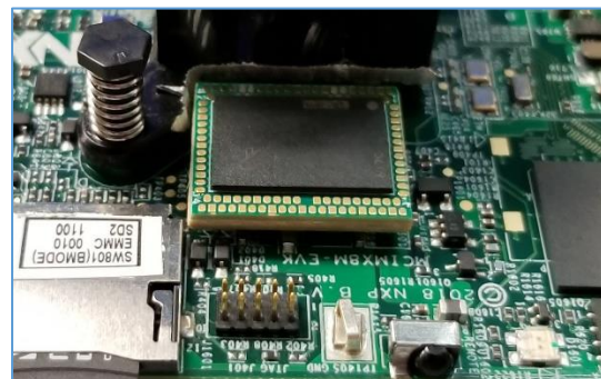
Figure 1 Direct Attach interposer installed under a memory component
