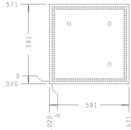
Figure 3 LPDDR4 272 Ball Riser Mechanical Dimensions
