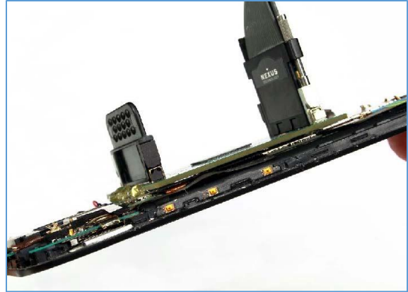
Figure 1 MA 5100 interposer installed under a memory component
