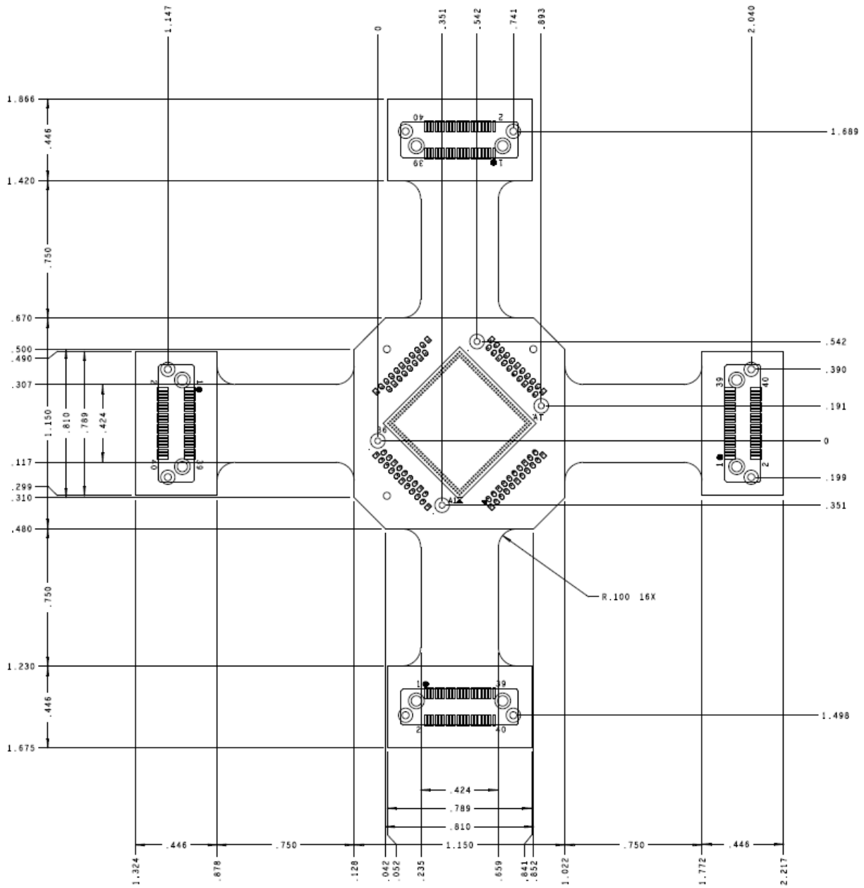
Figure 2 LPDDR4 272 Ball Compliance Interposer Mechanical Dimensions
