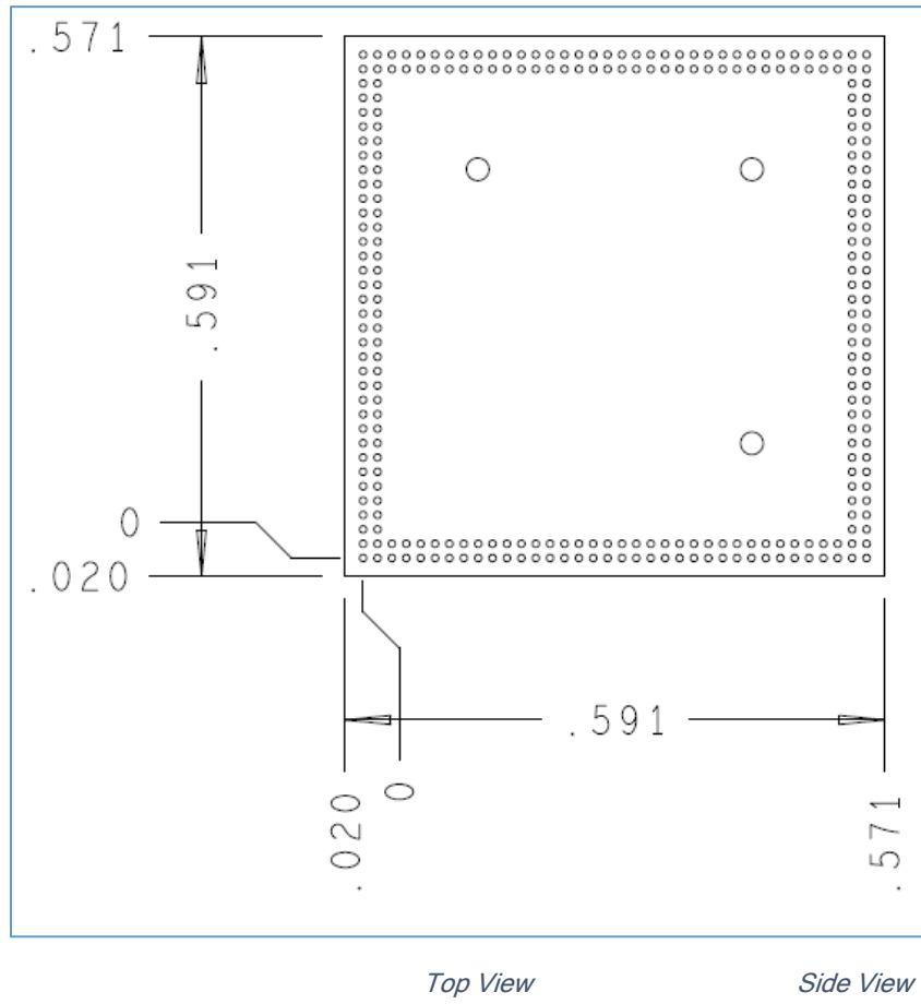
Figure 3 LPDDR4 272 Ball Riser Mechanical Dimensions
