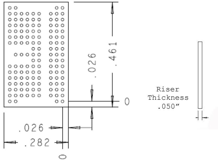
Figure 6: LPDDR2-134 ball Riser Dimensions
