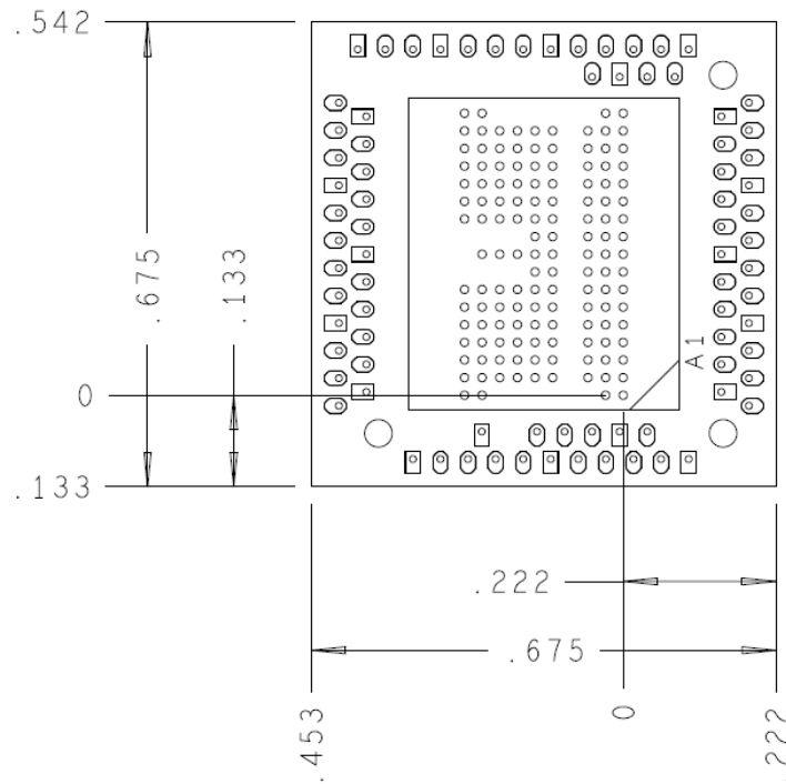
Figure 7: LPDDR2-134 Oscilloscope Component Interposer Dimensions
