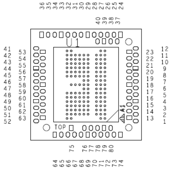
Figure 3 - Probe point locations top side
