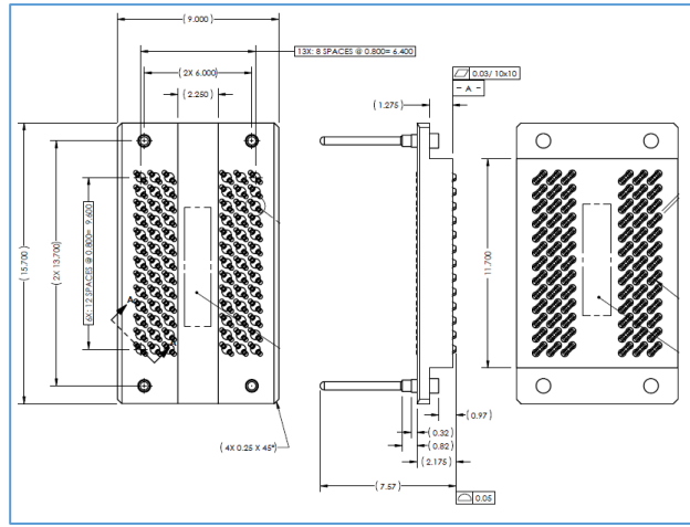
Figure 2 Interposer Socket Mechanical
