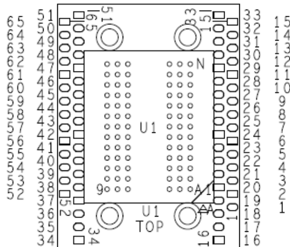
Figure 3 DDR4 78 Pin XH Series Socketed Interposer Probe Point Locations
