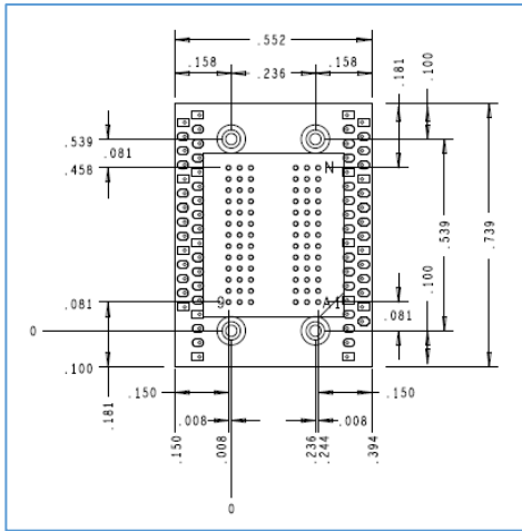
Figure 1 Interposer Mechanical
