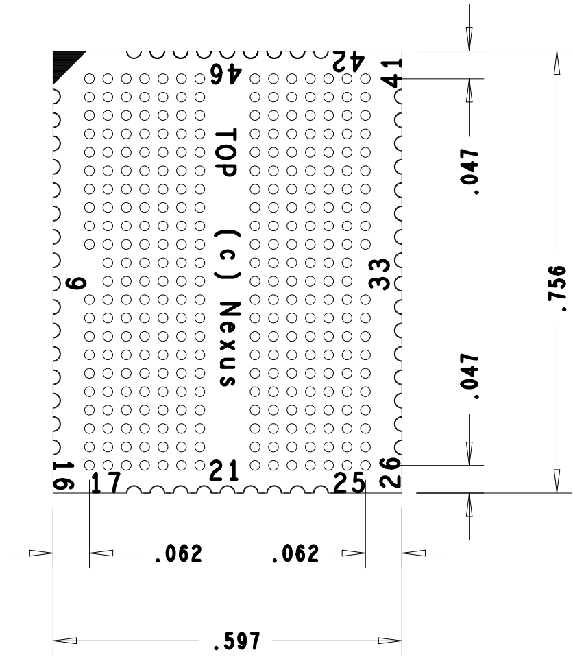
TOP VIEW
