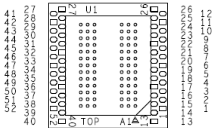
Figure 4 DDR5 Oscilloscope Interposer Direct Attach Probe Point Locations
