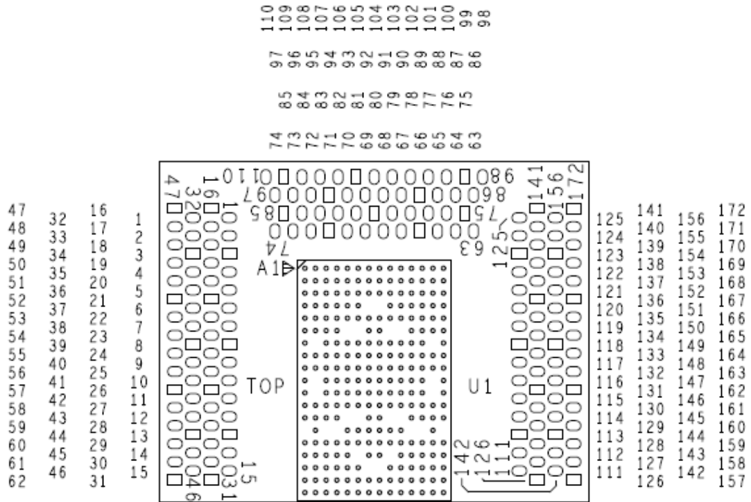
Figure 4 - DDR5 240 Ball XH Series RCD Oscilloscope Component Interposer Probe Point Locations
