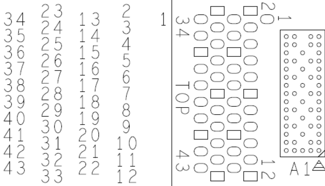
Figure 4 DDR5 DB01 XH Series Direct Attach Interposer Probe Point Locations
