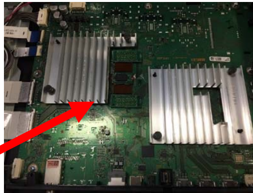
Working with the customer, it is agreed upon that the heat sink should be cut for interposer clearance. All work done by Nexus.
