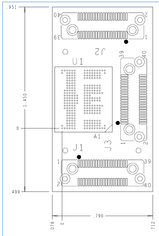
Figure 2 LPDDR4 254 Ball Compliance Interposer Mechanical Dimensions
