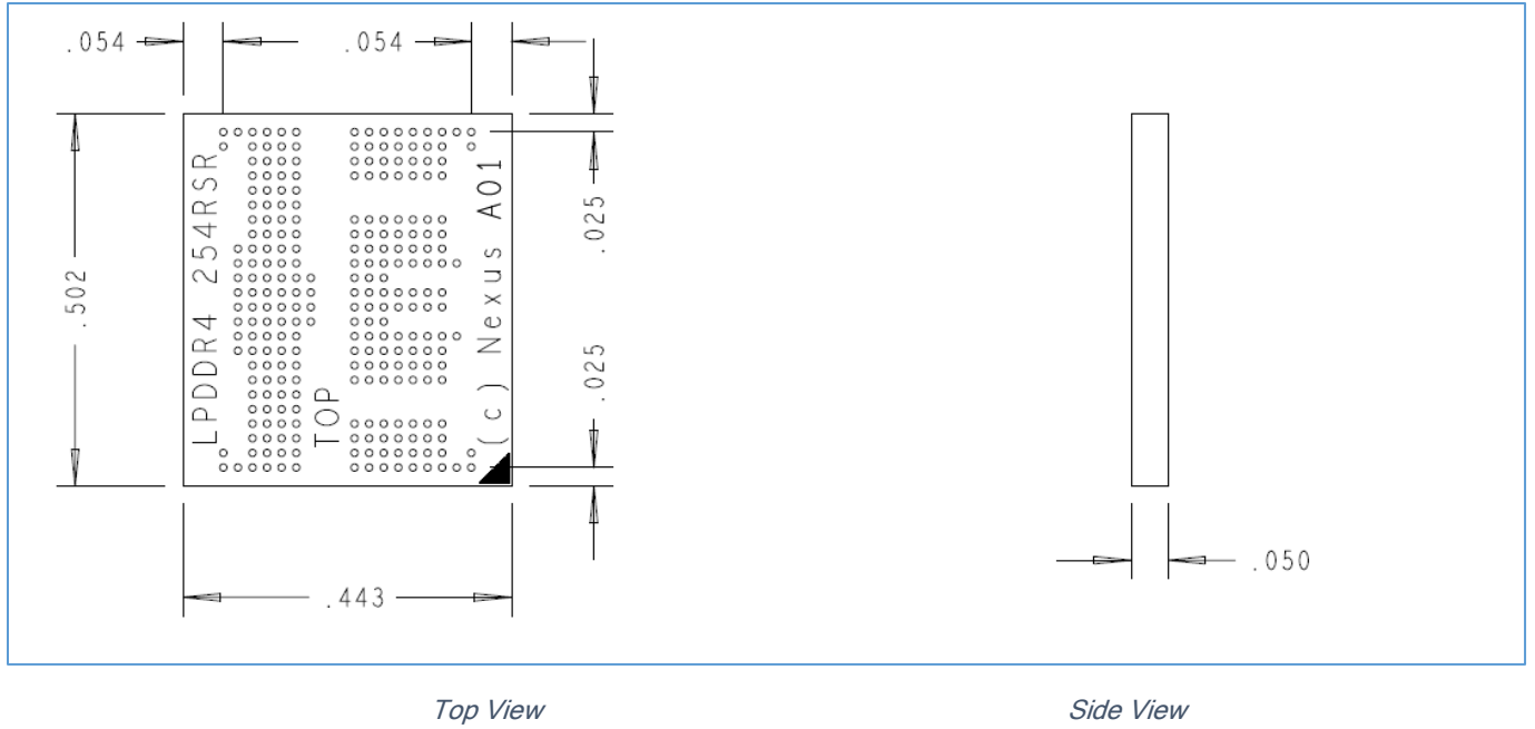
Figure 3 LPDDR4 254 Ball Riser Mechanical Dimensions
