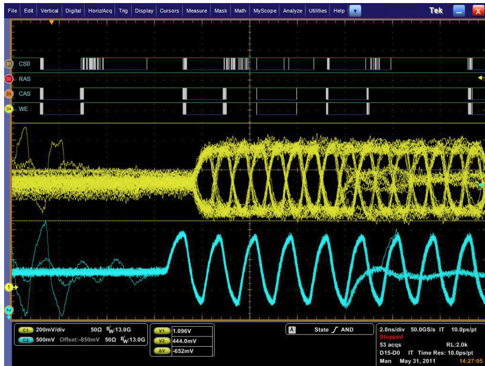
Figure 1 - MSO Display of the Analog/Oscilloscope DQ and DQS signals triggered on a write command using the digital probing provided by the DDR4 MSO SODIMM Interposer
