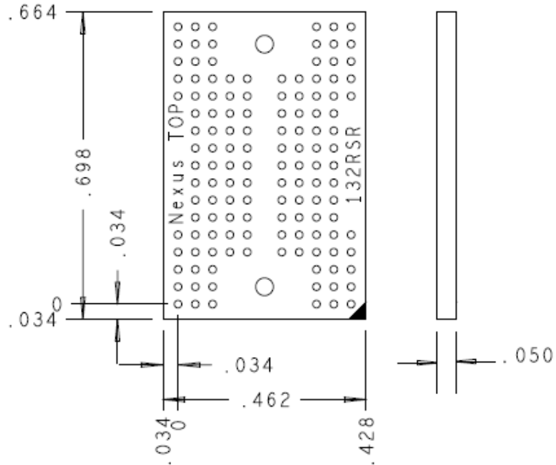
Top View Dimensions
