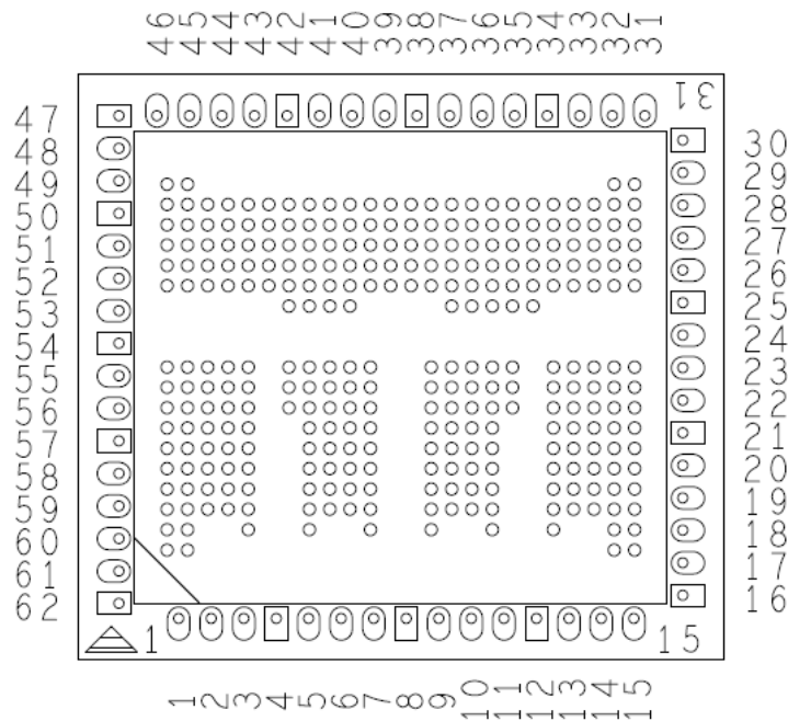
Figure 4 LPDDR5 297 Ball XH Series Direct Attach Interposer Probe Point Locations
