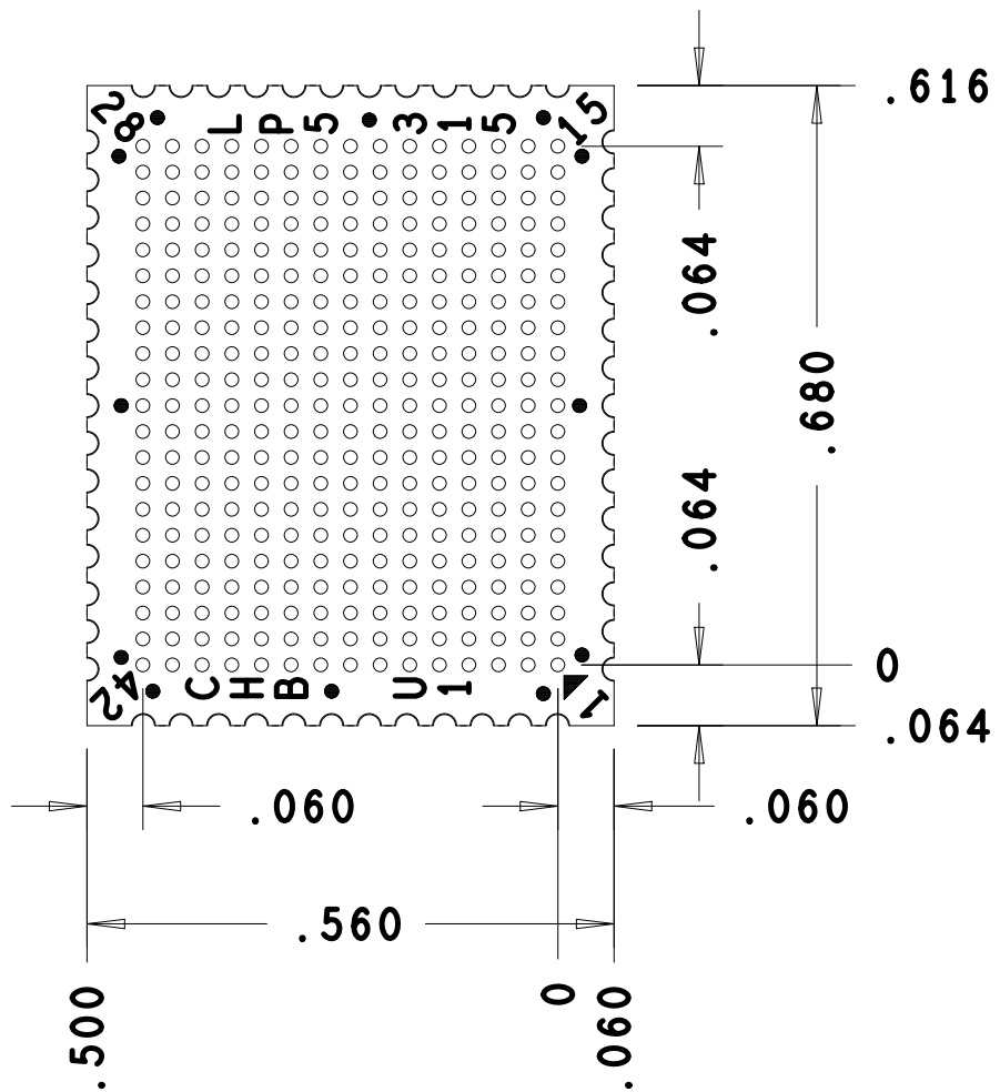
TOP VIEW
