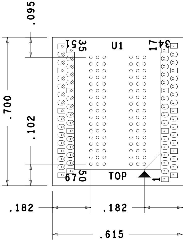
TOP VIEW
